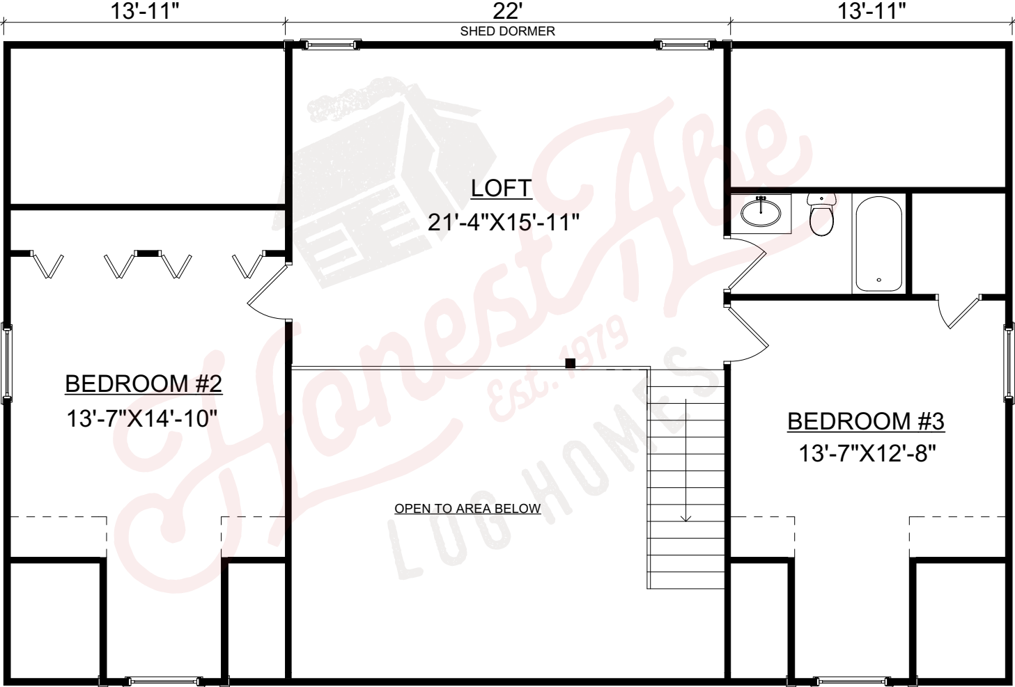
2 nd Floor
